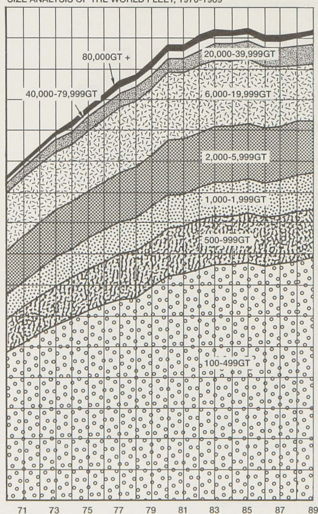
SIZE ANALYSIS OF THE WORLD FLEET, 1970-1989
