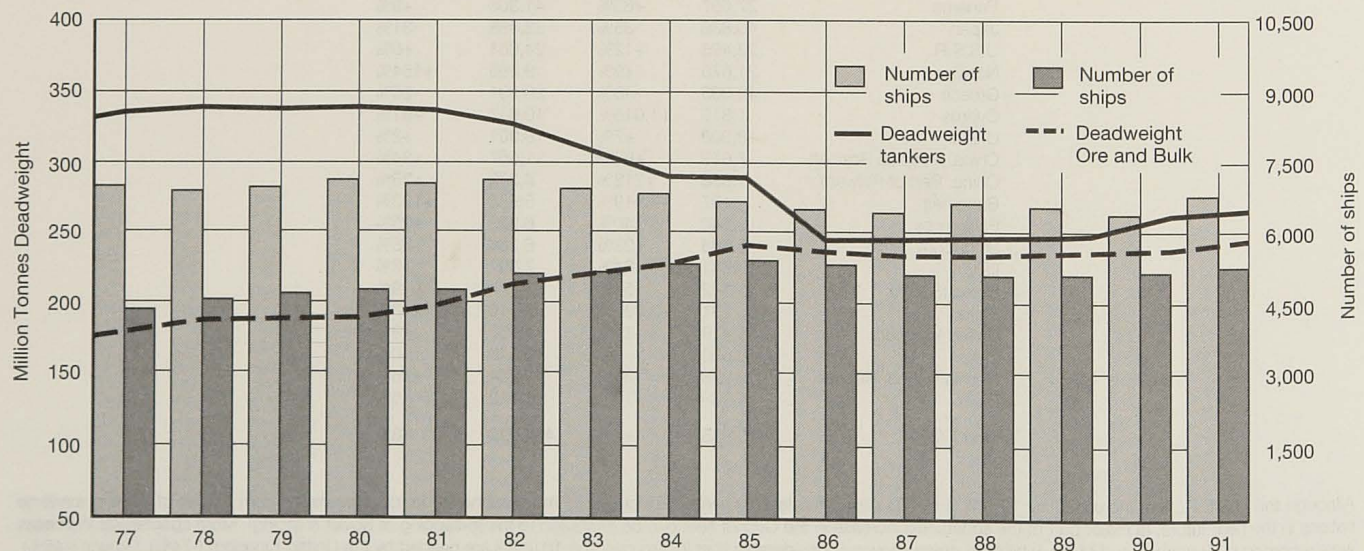
OIL TANKER AND ORE & BULK CARRIER FLEETS, 1977-1991
