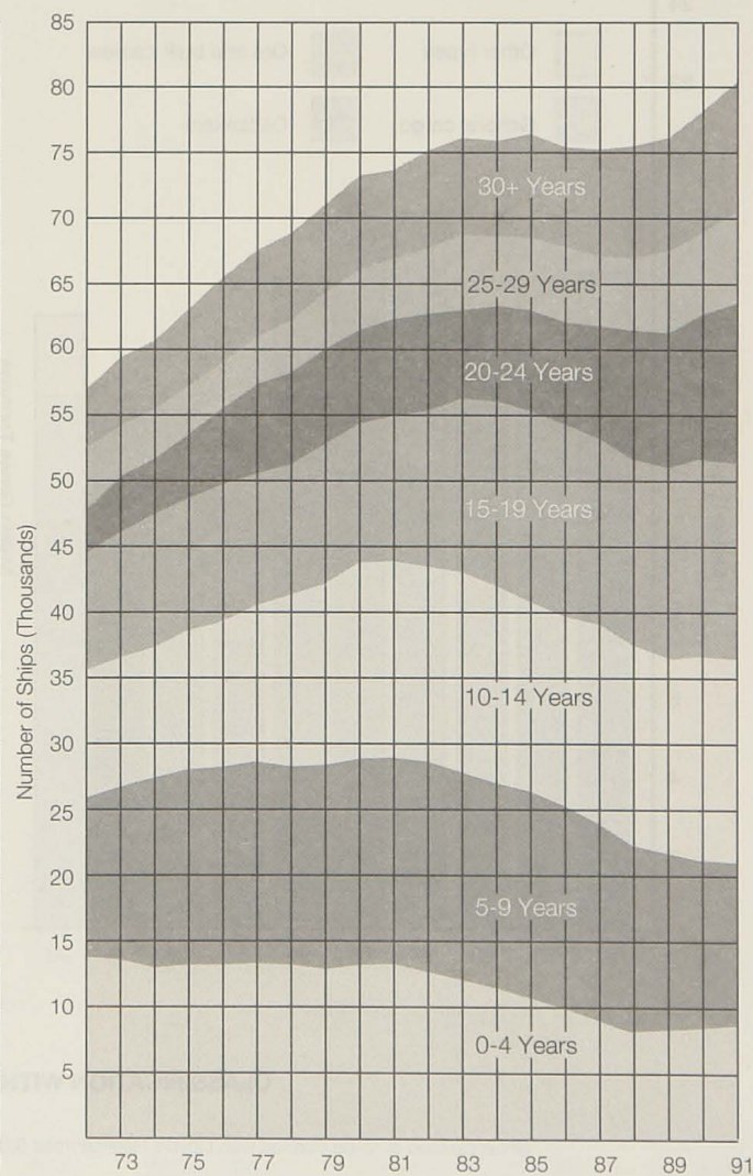
AGE ANALYSIS OF THE WORLD FLEET, 1972-1991
