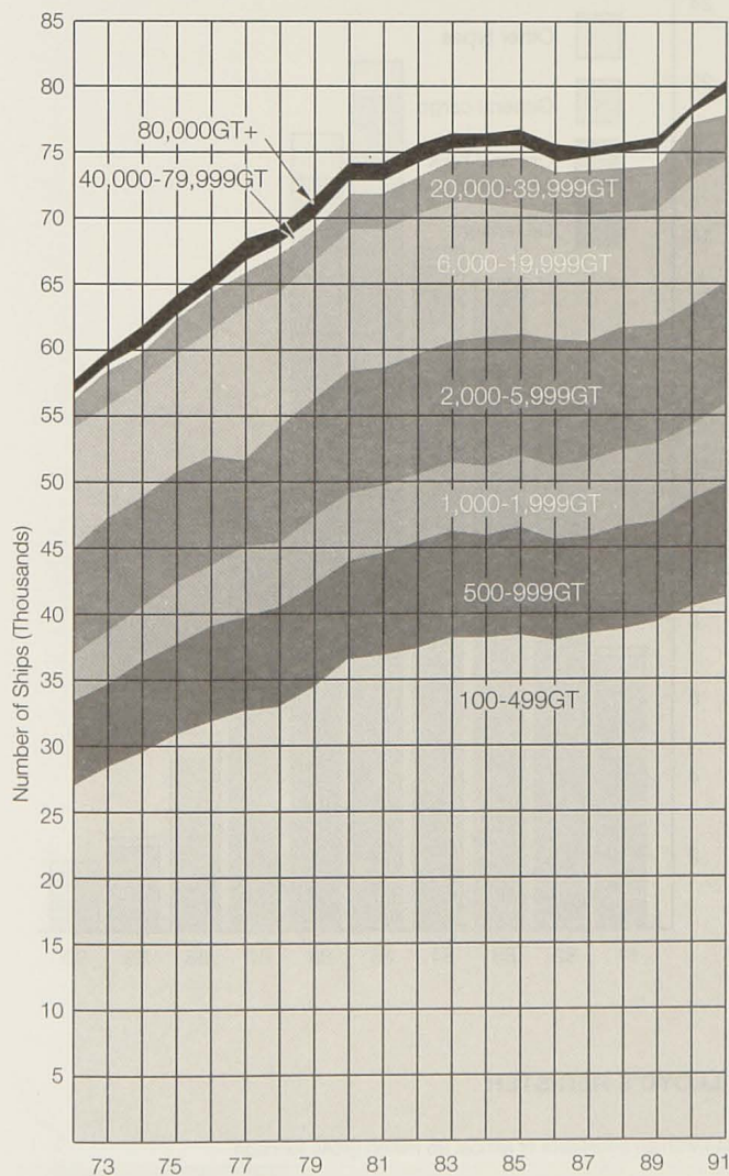
SIZE ANALYSIS OF THE WORLD FLEET, 1972-1991
